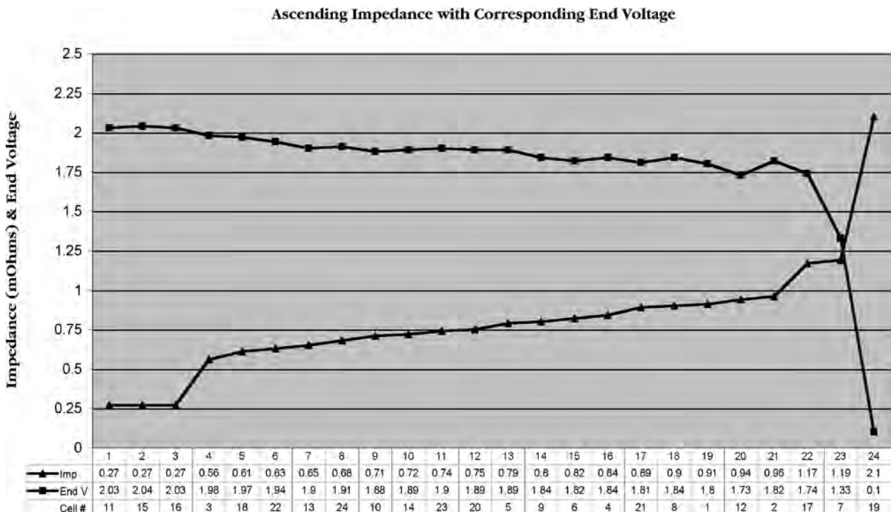
Figure 5 Ascending impedance with corresponding end voltage
